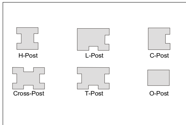
Fig. 12: Typical concrete post sections.
