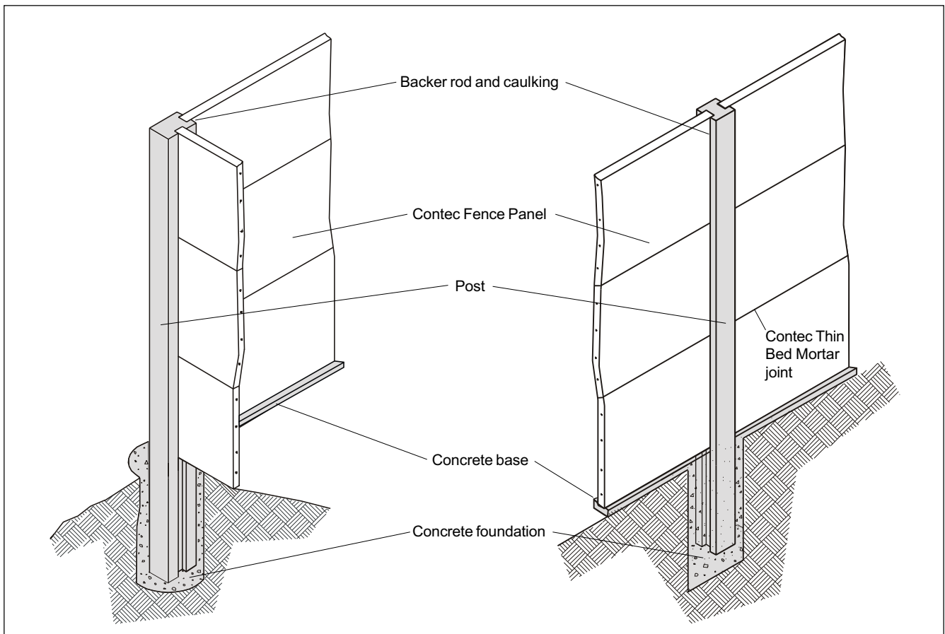
Fig. 2: Contec Fence System.
