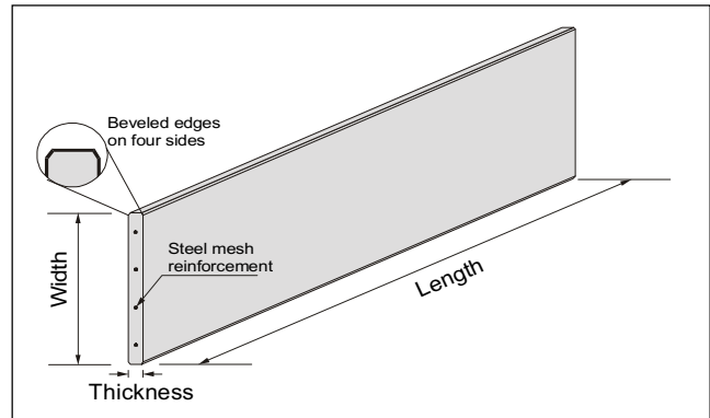
Fig. 1: Contec Fence Panel.
